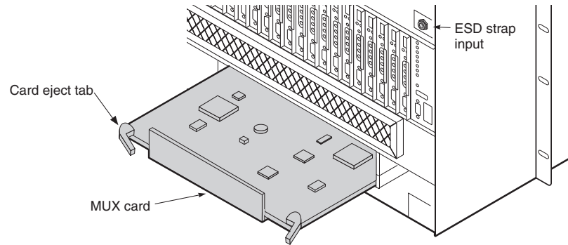
Figure 28. Installing an HXU-359
