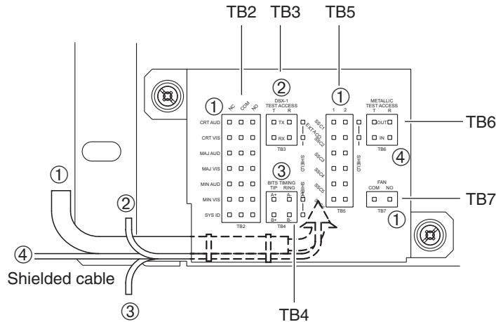
Figure 10. Common Access Panel
