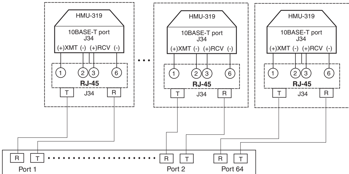
Figure 14. Multishelf 10BASE-T Configuration
