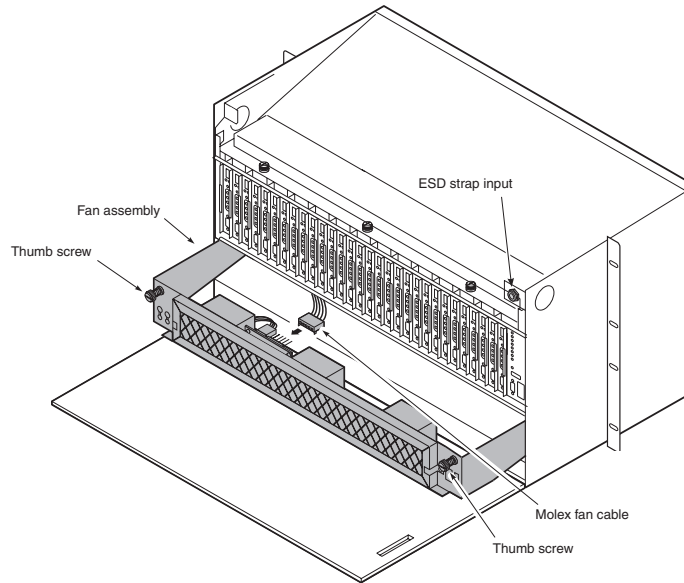
Figure 34. Installing the Fan Assembly (Cover Down)
