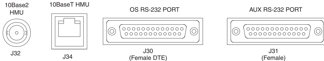
Figure 13. Network Interface Connections
